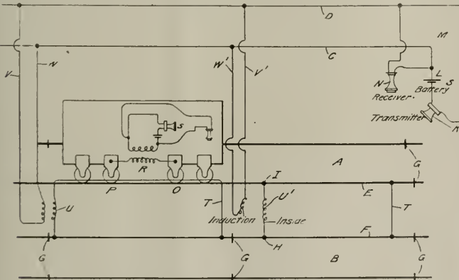
WIRING DIAGRAM—MACFARLANE TELEPHONE SYSTEM.
